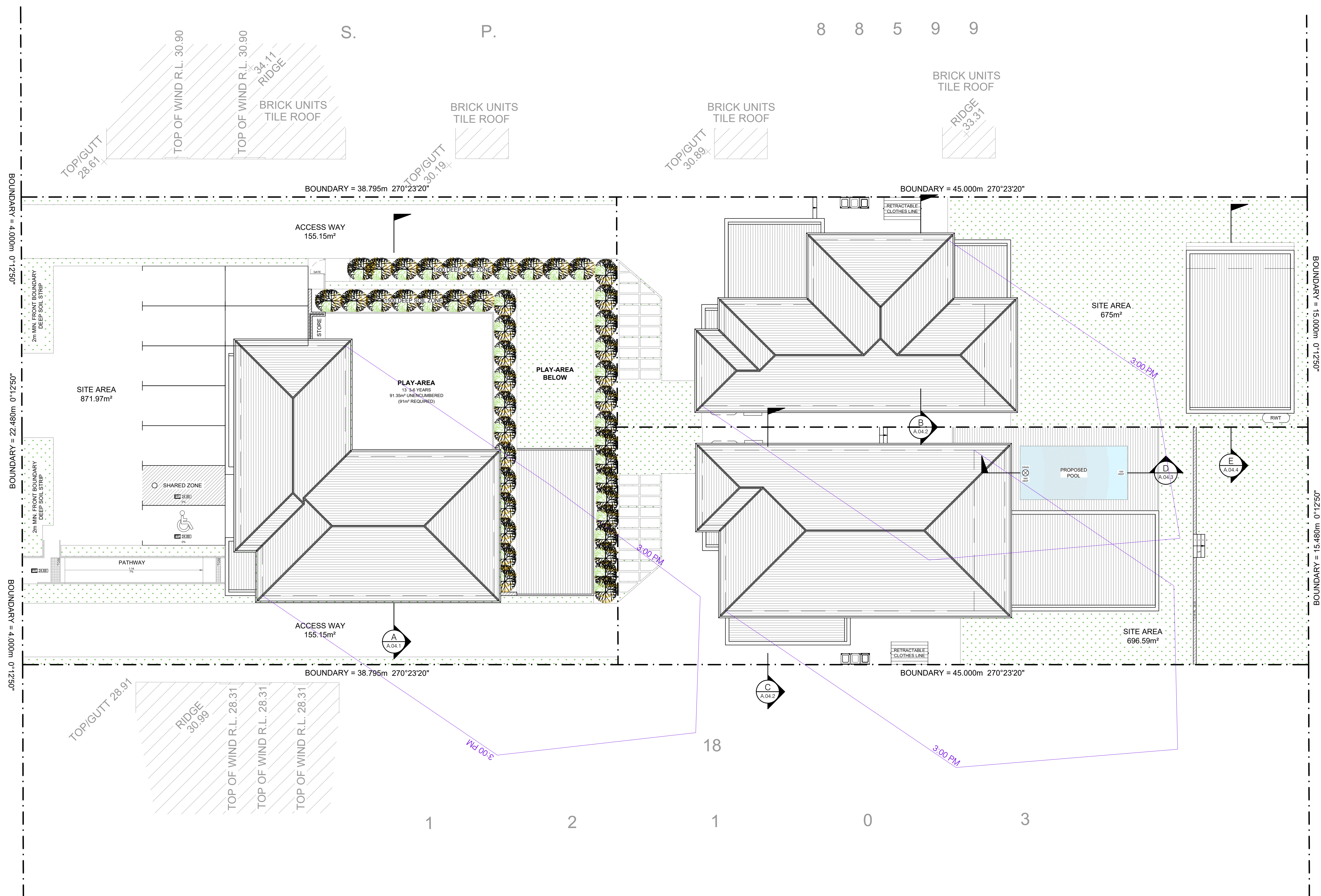
PROPOSED SHADOW DIAGRAM JUNE 21st 3PM SCALE - 1 : 250
